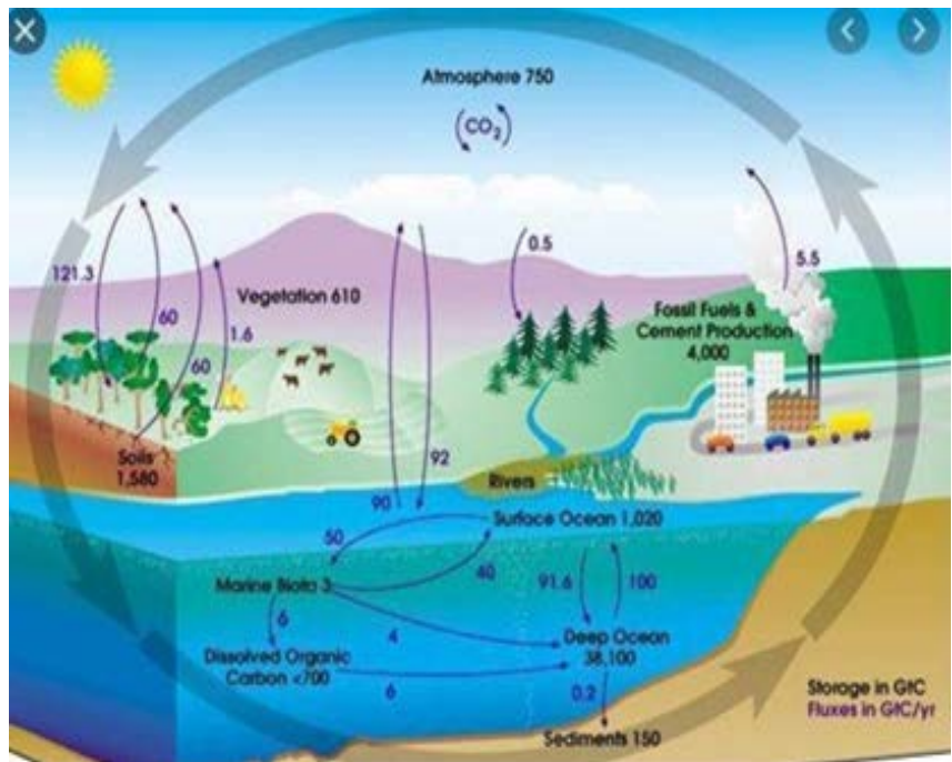
FIGURE 1 CARBON CYCLE
